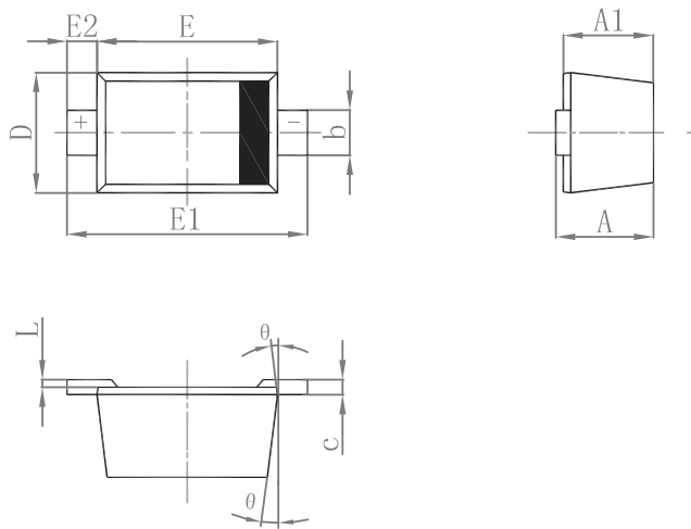
SOD-523 Package Outline Dimensions
